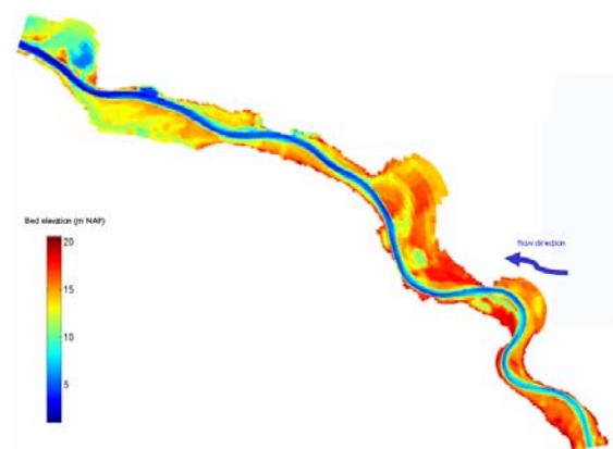
Figure 2. Morphological Delft3D model.
