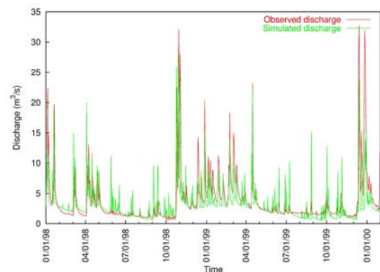
Figure 4. Hydrograph simulation.
