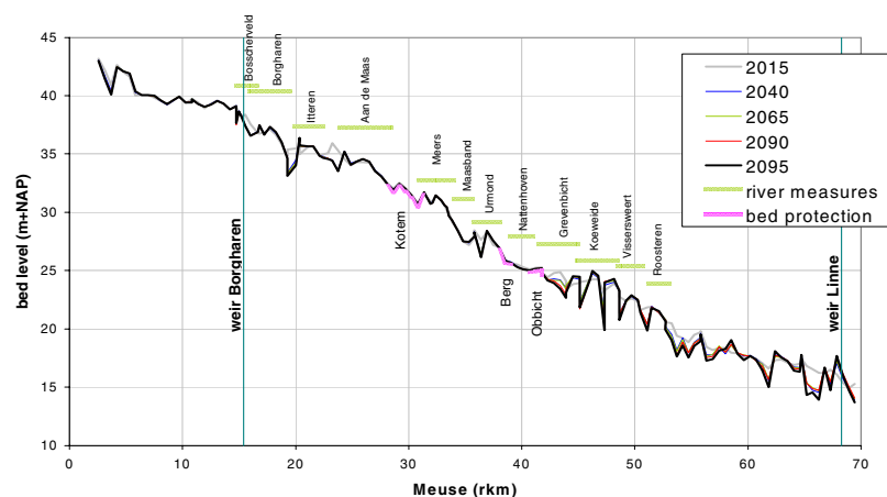
Figure 4. Riverbed development (Preferred Alternative, historical discharge scenario).
