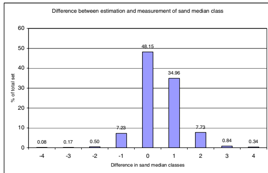
Figure 1. Differences between estimation of sand median class by descriptors TNO-NITG (from DINO) and grain size analysis of sand median class. X axis is expressed as total difference in sand median classes. For example: estimated median class: very fine sand, measured median class: very coarse sand, total difference in median classes is 3. With: -2/-1 estimated sand median class (from DINO) coarser than measured sand median class 0 no difference 1/2/3/4 measured sand median class (from DINO) coarser than estimated sand median class
