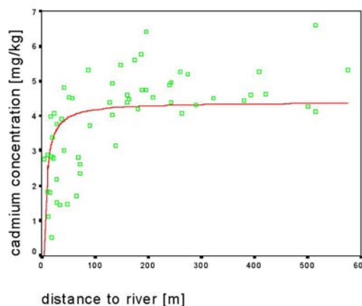
Figure 2. Relationship between distance to the river in the floodplain and the cadmium concentration of the sediment for all investigated floodplains and different inundation periods in 2001 and 2002.
