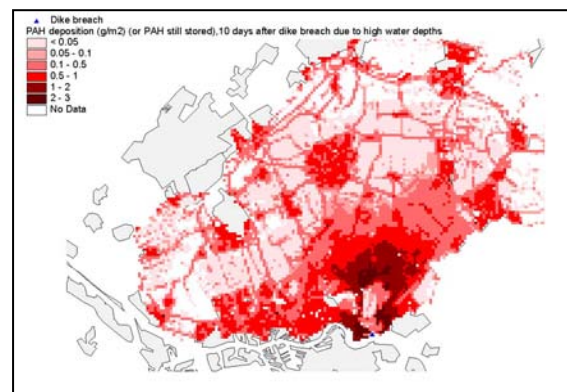
Figure 4. Concentrations of PAH's, present after 10 days, either deposited after release subject to the 'h' criterion, or as unreleased source.
