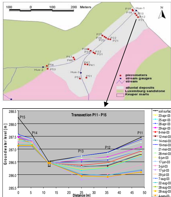
Figure 2. Fluctuation of piezometric level Huelebach catchment Apr. 2003 - Sep. 2003.
