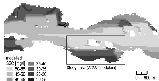
Figure 2. Modelled suspended sediment concentrations in the model area. The box denotes the same area as shown in Figure 3.
