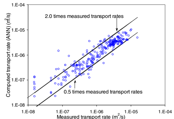
Figure 1. A comparison of the total transport rates predicted by the ANN model with the measured transport rates.
