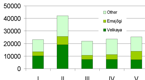
Figure 7. Simulated Ntot loads (T/yr) for 1985 - 1999 and five future scenarios.
