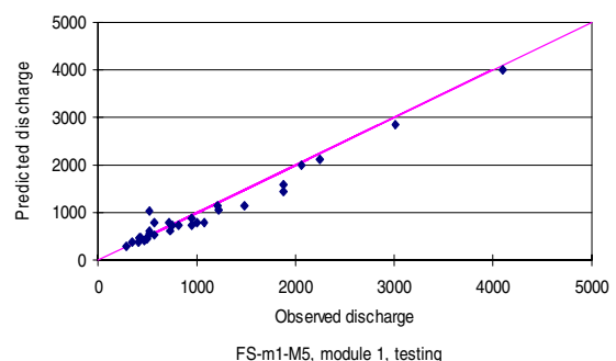
flood season (samples with QX_{t-1} > 1000 \text{ m}^3/\text{s} ). An increase of accuracy can be observed.
