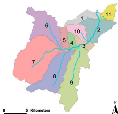
Figure 1. Hesperange sub-catchment sub-divided in REW's.
