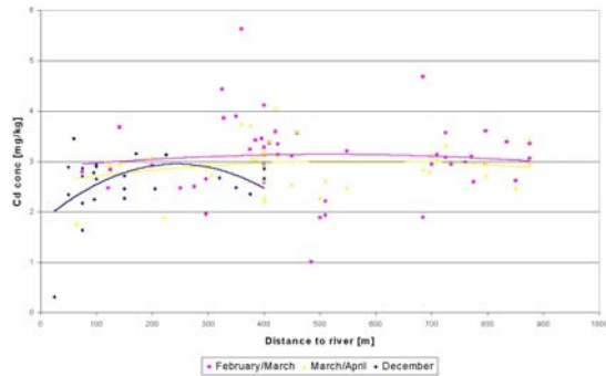
Figure 3. Cadmium concentration of the sediment against distance to the river in the Afferdensche en Deestsche Waarden for three inundation periods in 2001 and 2002.
