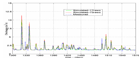
Figure 4. Comparison of simulated and measured discharges at outlet of Geer river.
