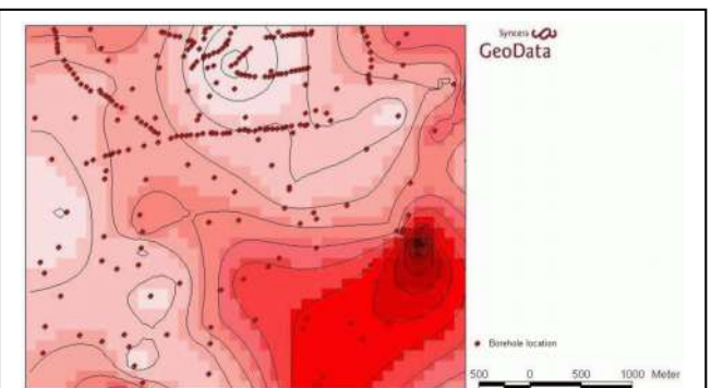
Figure 1. Depth of the top of the coarse sand deposits belonging to the Kreftenheye Formation in the Tiel area along the river Waal.
